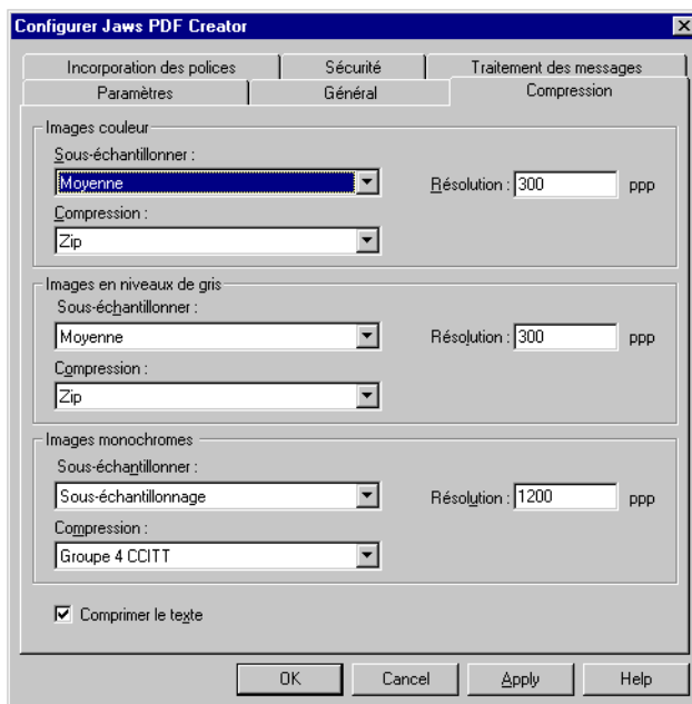
Figure 5.7 L'onglet Compression
